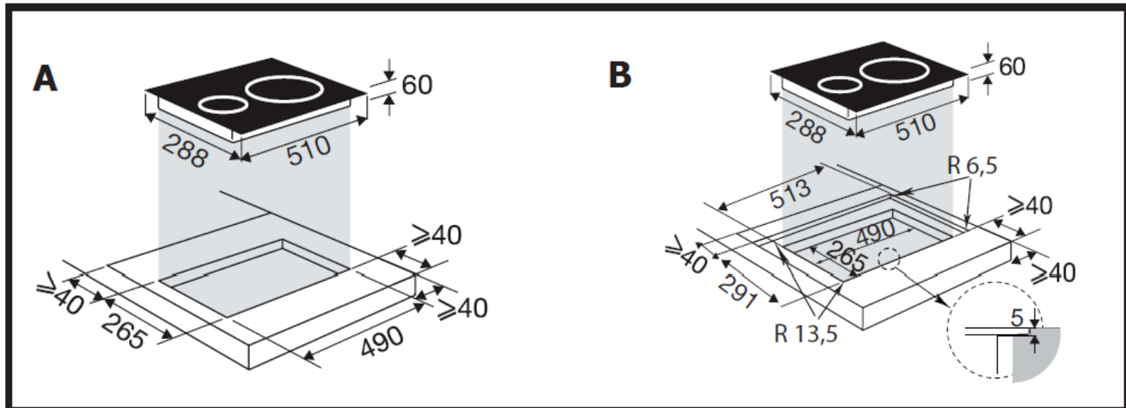
Fitting into the worktop
