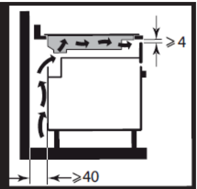
Fitting flush with the worktop
