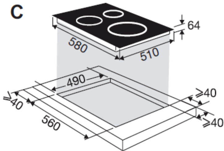
Fitting into the worktop
