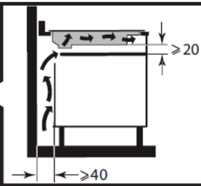
Fitting flush with the worktop
