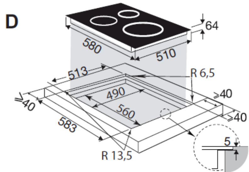
Fitting flush with the worktop
